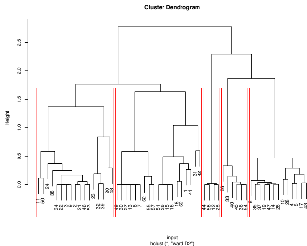
Figure 3: N-Gram Clustering Dendrogram of Facebook usage for a user
