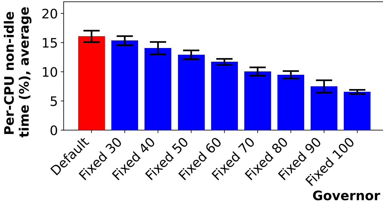
Little CPUs
